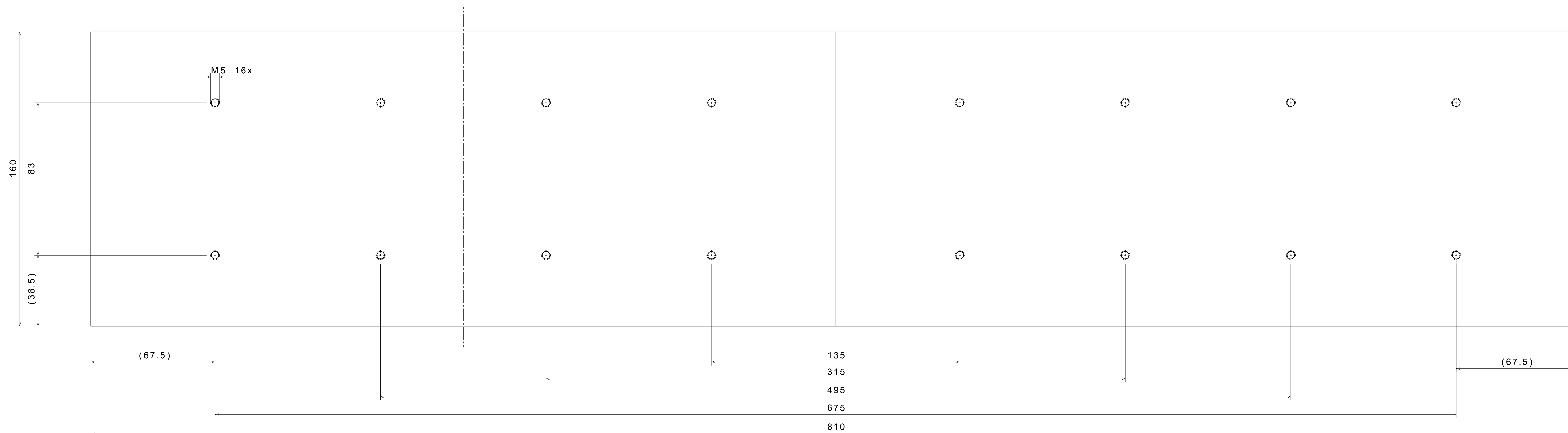
Bohrvorlage für CrossBoard® 11405A 2x drilling template for Cross Board® 11405A 2x
